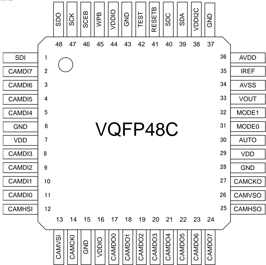
Fig.4 Pin configurations
