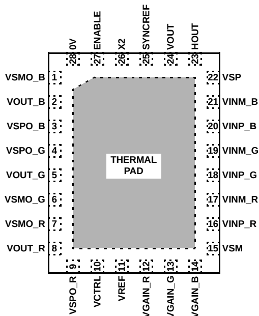
EL9111 (28 LD QFN) TOP VIEW
