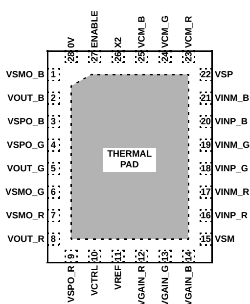
EL9112 (28 LD QFN) TOP VIEW
