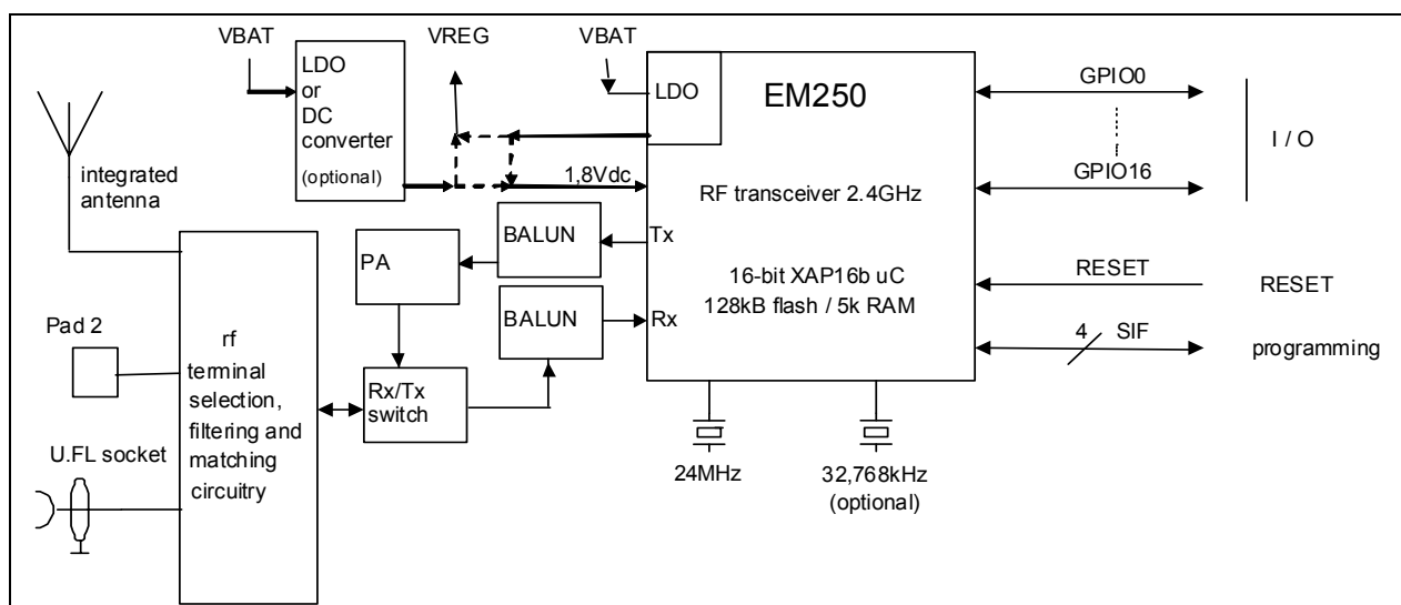
Figure 2: Hardware Diagram
