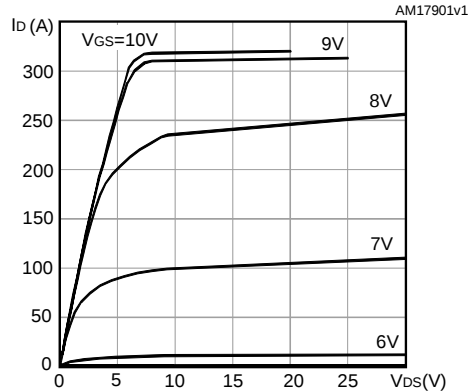
Figure 4: Output characteristics
