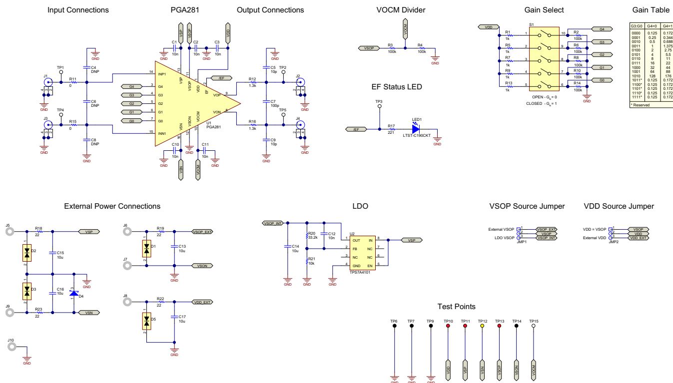
Figure 2. PGA281EVM Schematic
