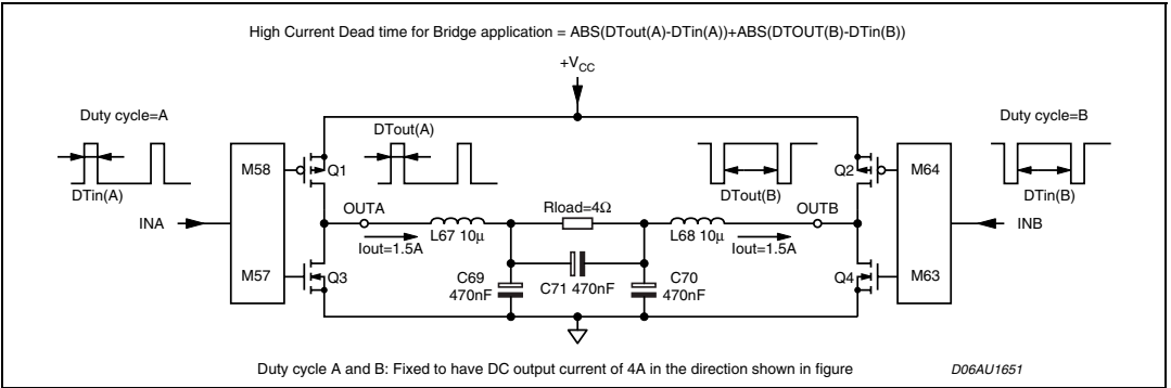
Figure 8. Test circuit 2
