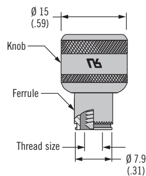
Press-In Style
