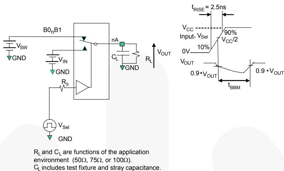
Figure 9. Break-Before-Make Interval Timing
