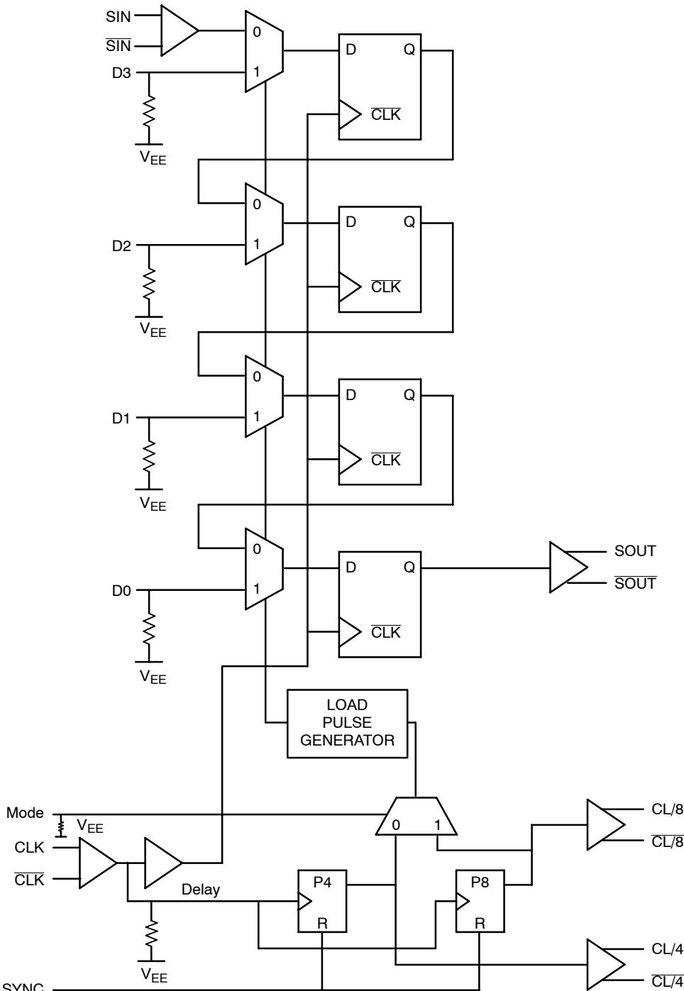
Figure 2. Logic Diagram
