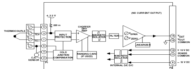
Figure 1. 3B47 Functional Block Diagram
