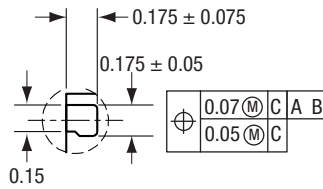
Detail B Scale: 2X 1X This Rotation 1X Rotated 180°
