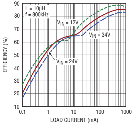
Efficiency ( V_{OUT} = 5V , SYNC = 0V)
