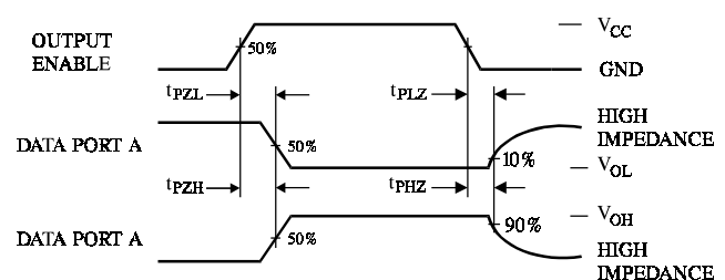
Figure 5. Switching Waveforms
