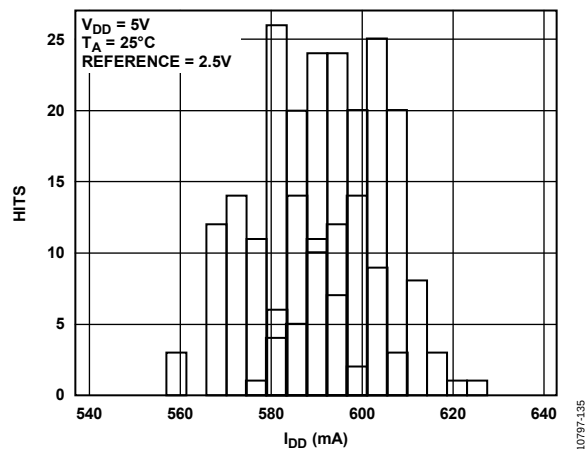
Figure 22. I_{DD} Histogram
