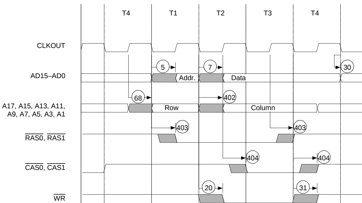
Figure 32. DRAM Write Cycle without Wait States Waveform
