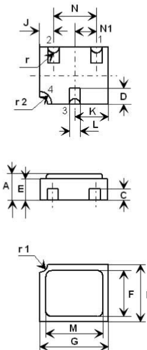
Figure 4. UB package outline
