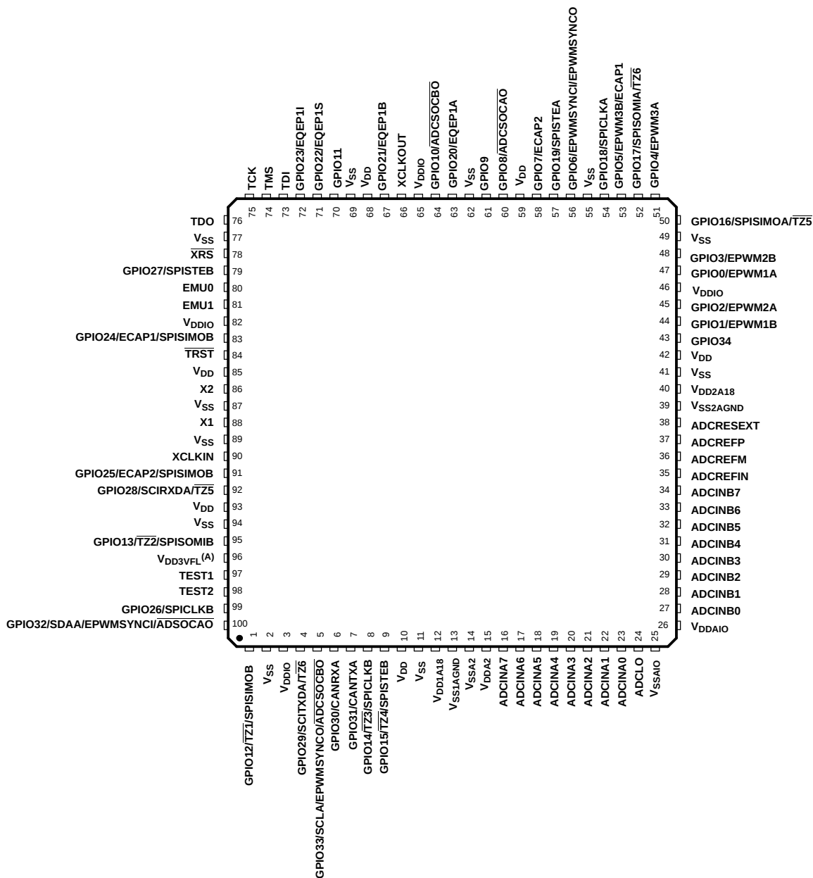
Figure 2-3. TMS320F2802, TMS320F2801/UCD9501, TMS320C2802, TMS320C2801 100-Pin PZ LQFP (Top View)
