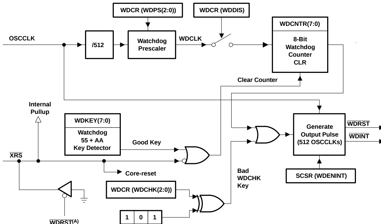
Figure 3-13. Watchdog Module
