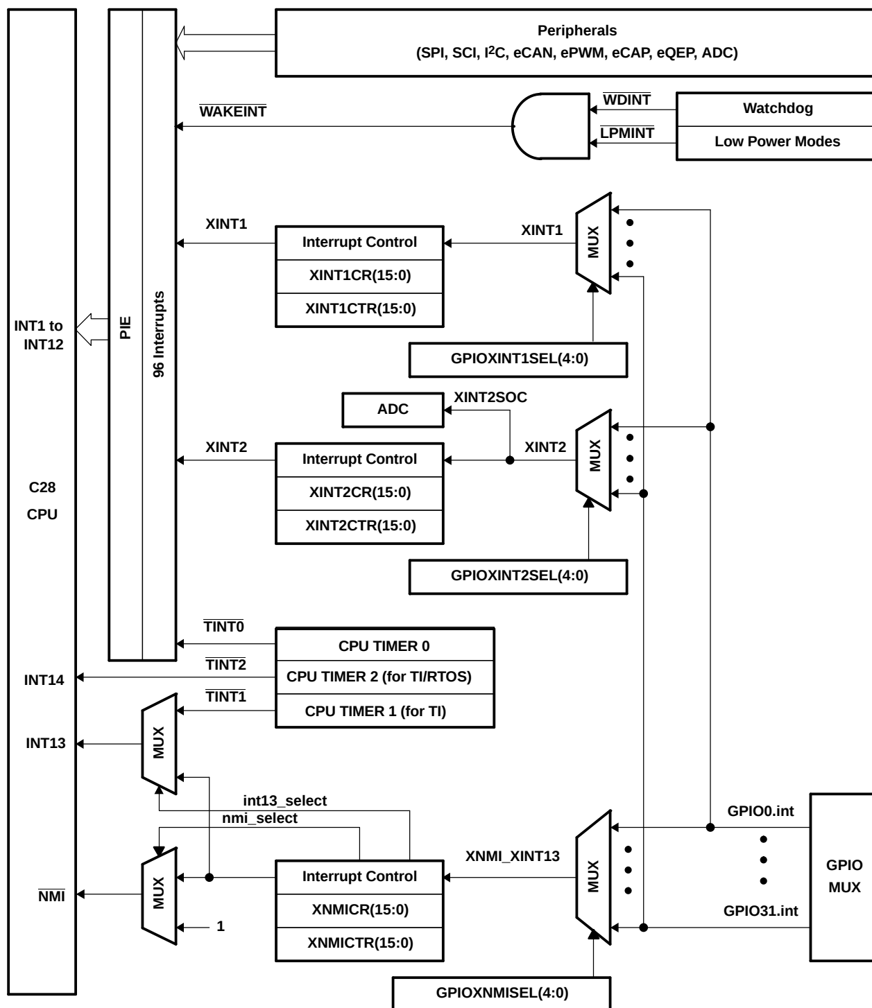
Figure 3-6. External and PIE Interrupt Sources
