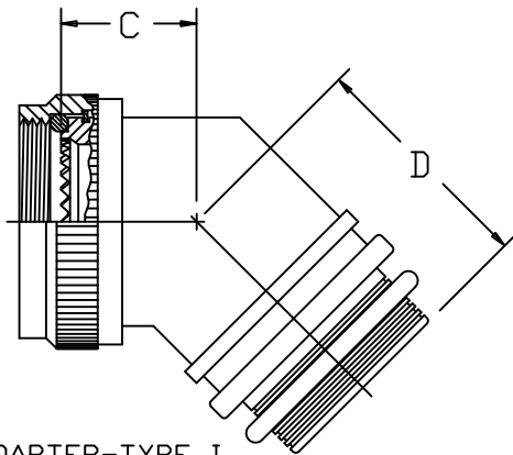
45° ADAPTER-TYPE I
