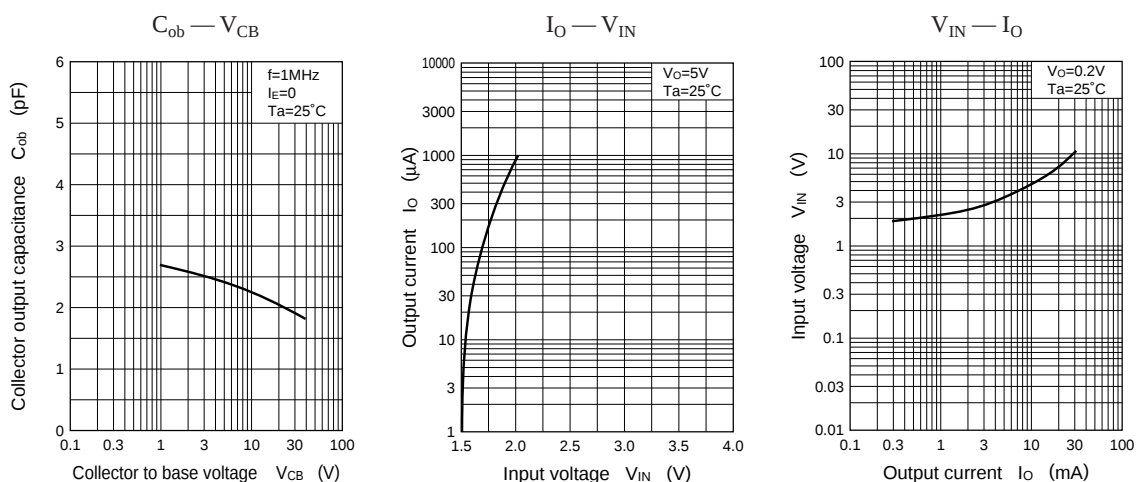
Characteristics charts of UN521F
