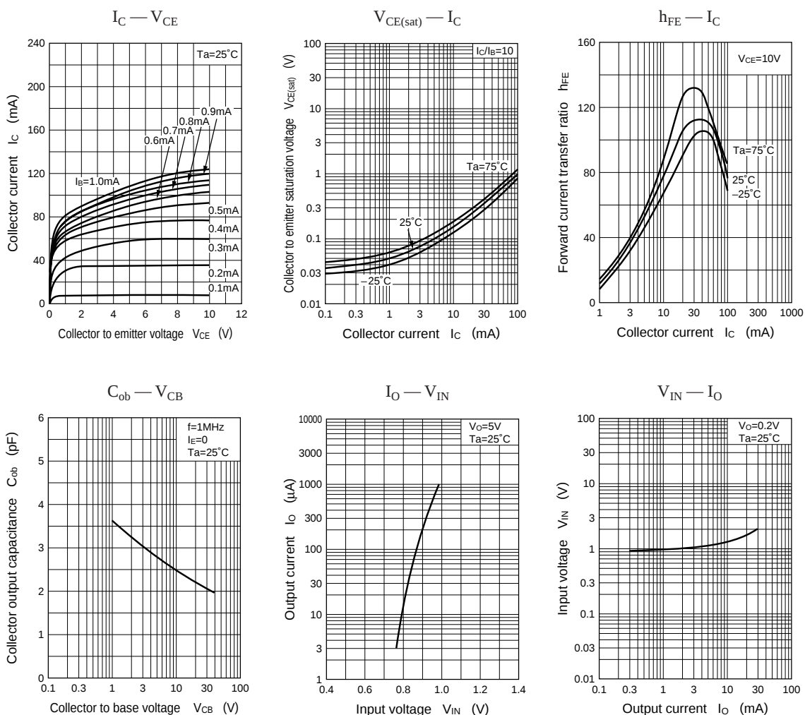
Characteristics charts of UN521F
