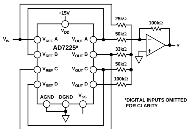
Figure 21. Complex Waveform Generation
