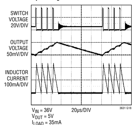
Operating Waveforms
