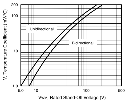
Figure 12. Breakdown Voltage Temperature Coefficient Curve
