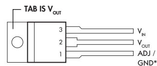
P PACKAGE (Top View)
