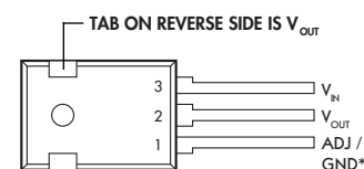
V PACKAGE (Top View)
