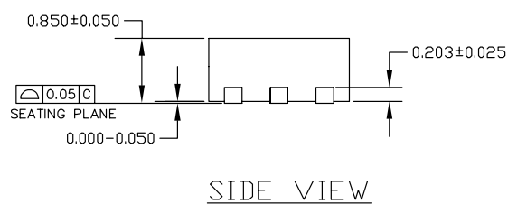
6-Pin 2x2 MLF® (ML)
