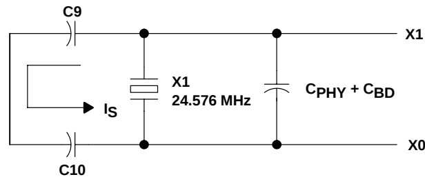
Figure 8–4. Load Capacitance for the TSB43AB21 PHY
