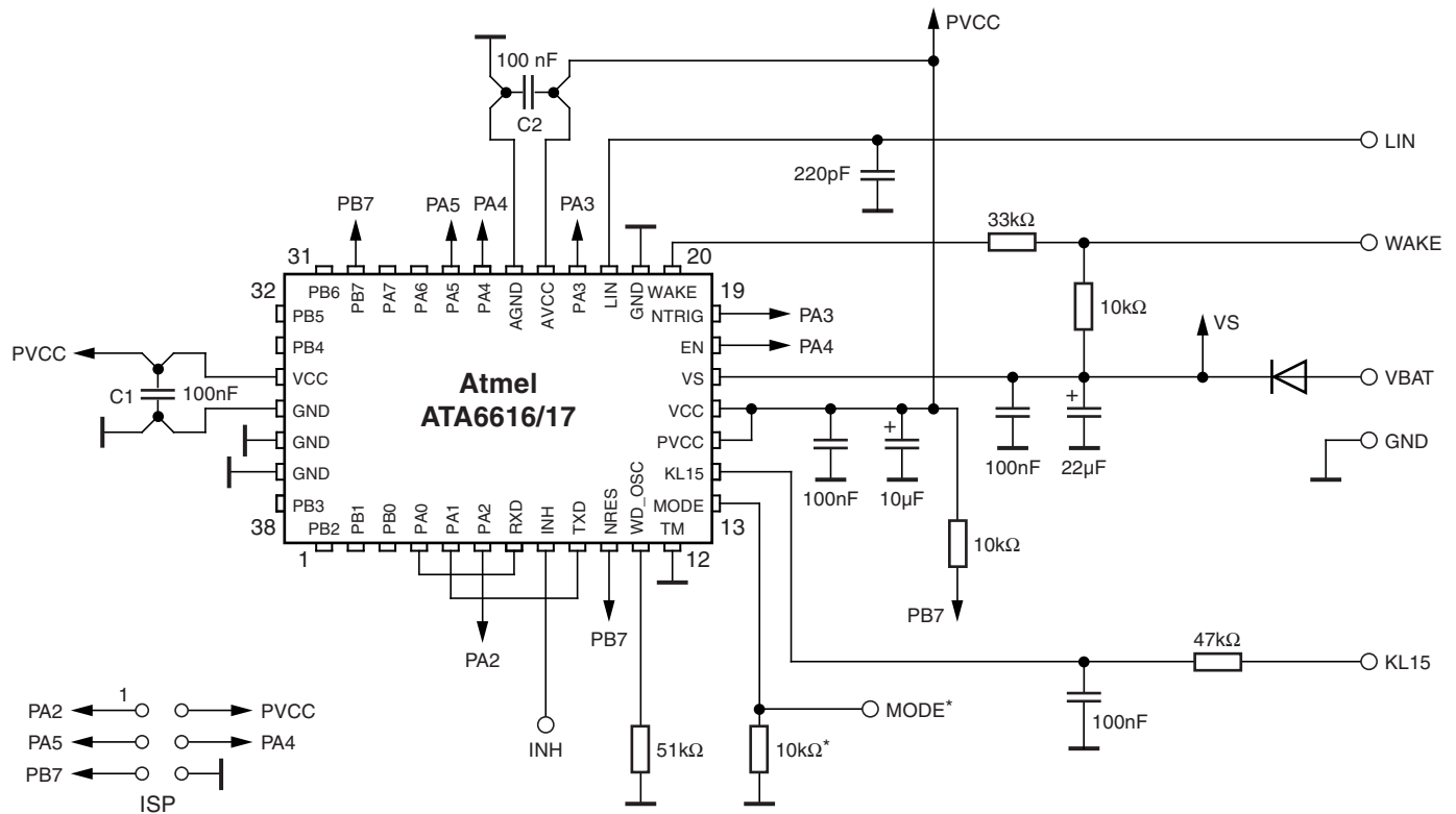
Figure 5-1. Typical LIN Slave Application
