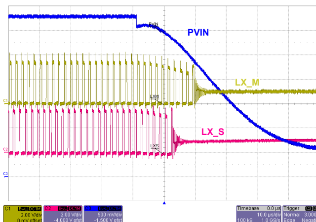
FIGURE 17. FALLING PVIN to M/S DISABLE
