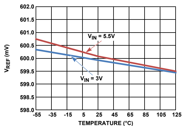
FIGURE 7. REF VOLTAGE vs V_{IN}
