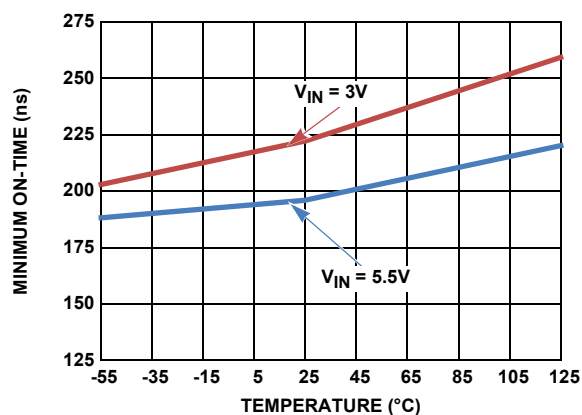
FIGURE 9. LXx MINIMUM ON-TIME vs V_{IN}
