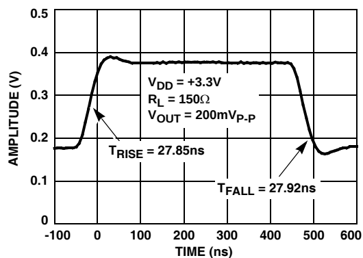
FIGURE 12. SMALL SIGNAL STEP RESPONSE
