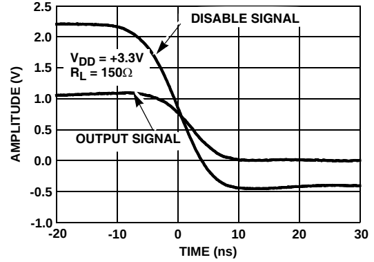
FIGURE 14. DISABLE TIME
