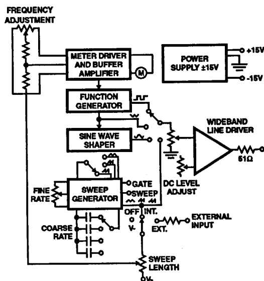
(C) INTERCONNECTIONS
