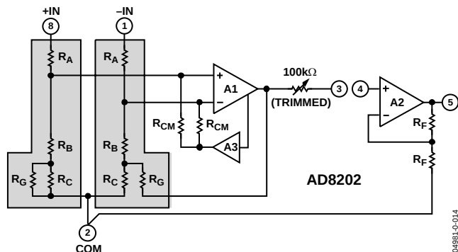
Figure 14. Simplified Schematic
