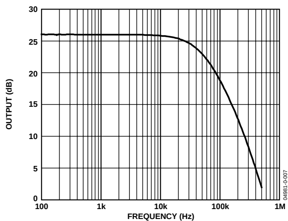
Figure 7. AD8202 Bandwidth
