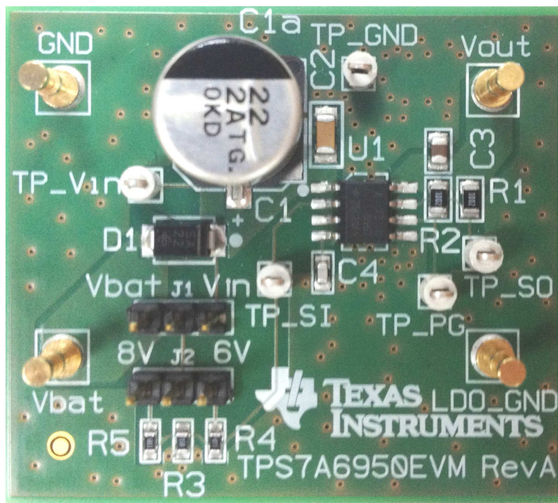
Figure 1. TPS7A69xxEVM Board
