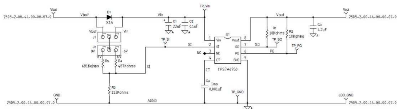
Figure 5. TPS7A69xx EVM Schematic
