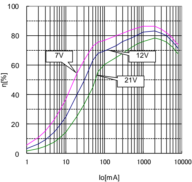
Figure 20. Efficiency (Vo= 1V, QLLM)
