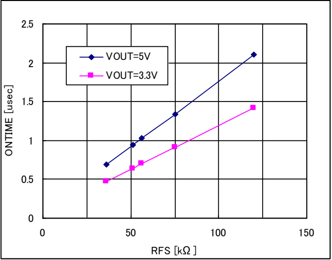
Figure 46. On time-RFS
