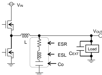
Output Capacitor
