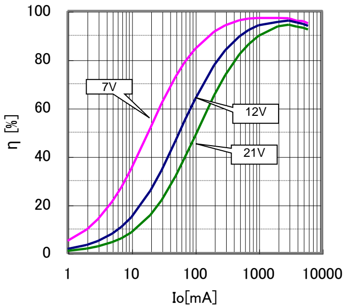
Figure 13. Efficiency ( V_o = 5V , PWM)
