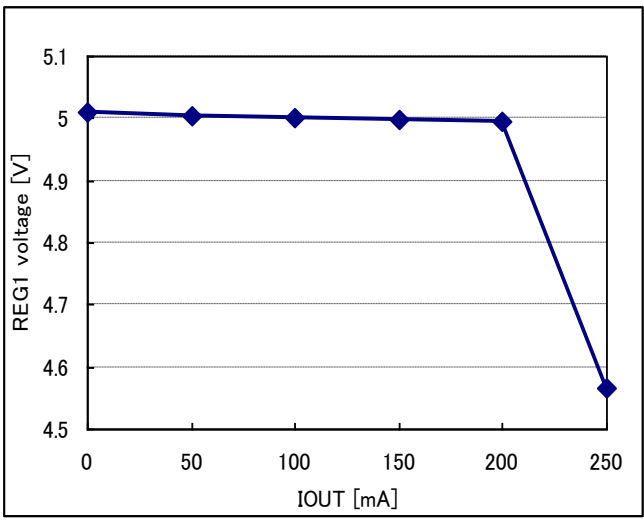
Figure 50. REG1 Load Regulation
