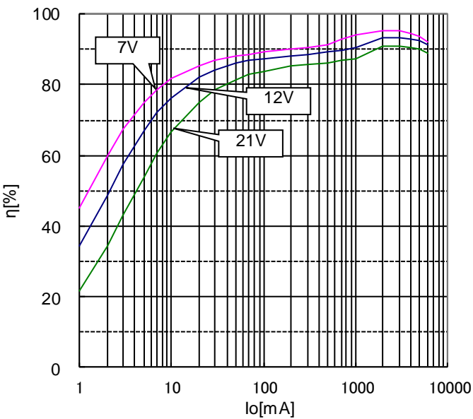
Figure 18. Efficiency (Vo= 3.3V, SLLM)
