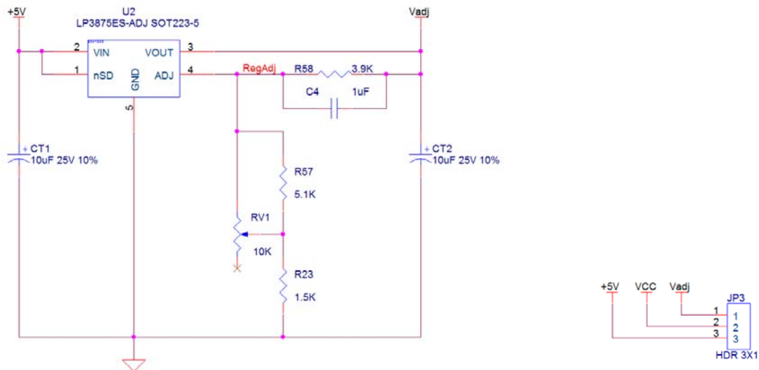
Figure 3-1. Schematics
