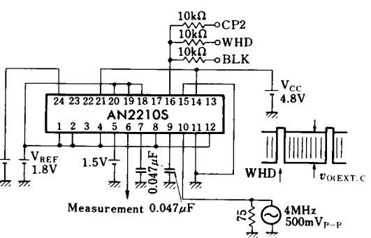
Test Circuit 6 ( v_{O(EXT.C)} )
