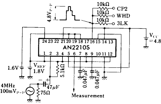
Test Circuit 4 ( v_{O(Chroma)} , G_{V(CC)} )
