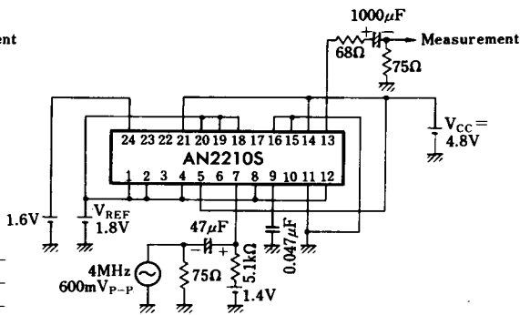
Test Circuit 10 (v O(6dB) )
