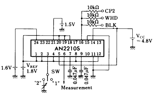
Test Circuit 3 ( v_{O(Main.Nega.)} , v_{O(Nega.-Ped.)1} , v_{O(Nega.-Ped.)2} )
