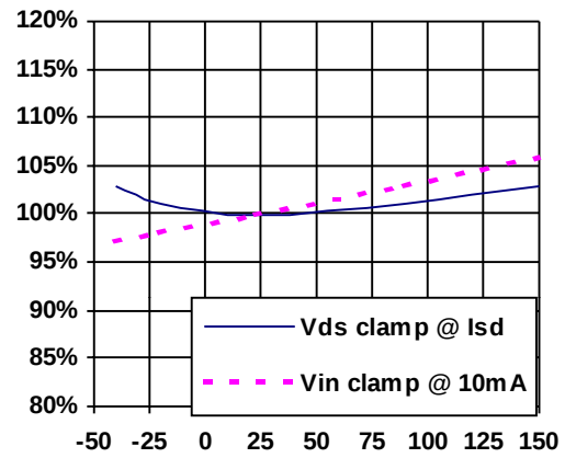
Figure 18 - Vin clamp and Vds clamp (%) Vs T_j ( ^{\circ}\text{C} )
