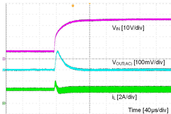
Figure 8-9. Line Transient
