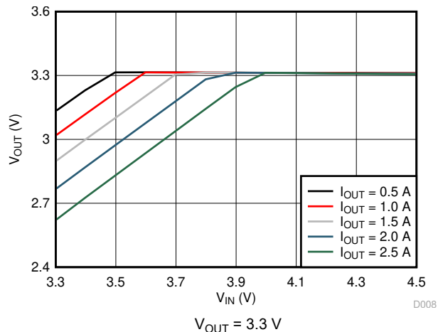
Figure 6-8. Dropout Curve
