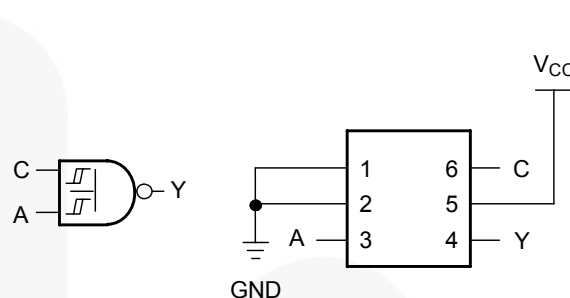
Figure 4. 2-Input NAND Gate
