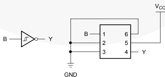
Figure 9. Inverter
