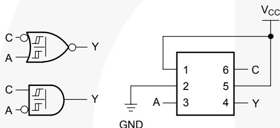
Figure 5. Input NOR Gate with One Inverted Input 2-Input AND Gate with One Inverted Input
