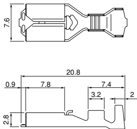
SPS-21T-250S
