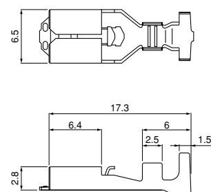
SPS-51T-205 (for 0.8 mm thick tabs)
