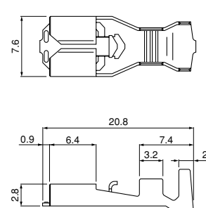
SPS-91T-250
