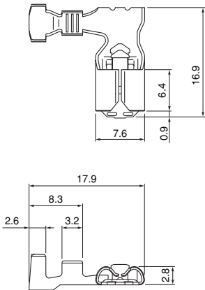
SFPS-61T-250H
