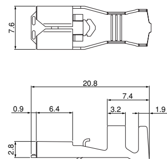
SPS-91T-250R
