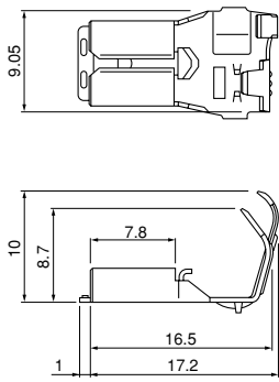
SFPS-61T-250
