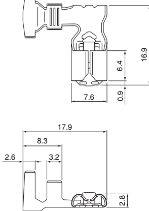
SFPS-91T-250H
