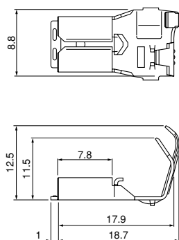
SFPS-91T-250
