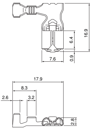
SFPS-21T-250H
