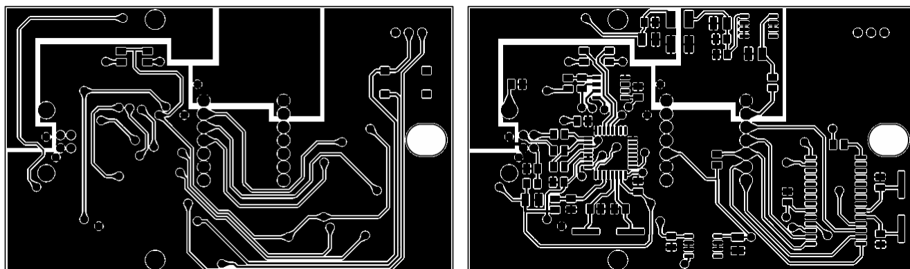
Figure 15. SCP1000 demo USB interface board PCB layout (left, top / right, bottom ).
