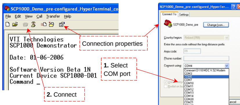
Figure 11. Windows HyperTerminal with SCP1000 demo info text.
