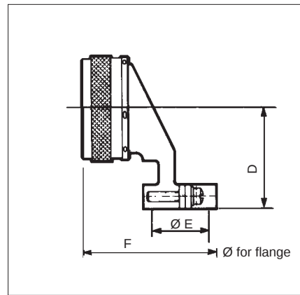
Elbow cable clamp type 03
