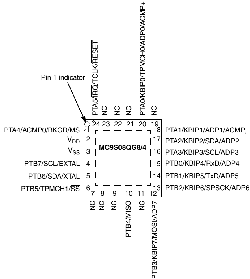
Figure 2-3. 24-Pin Packages
