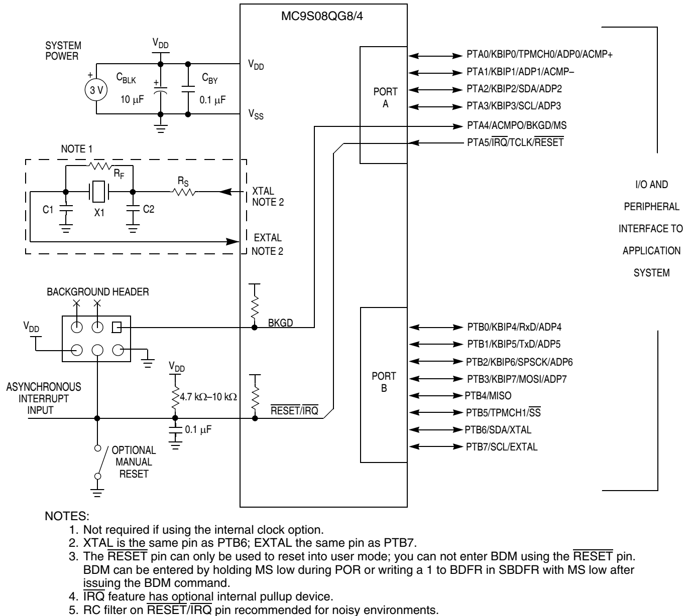
Figure 2-4. Basic System Connections
