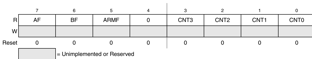
Figure 17-9. Debug Status Register (DBGS)
