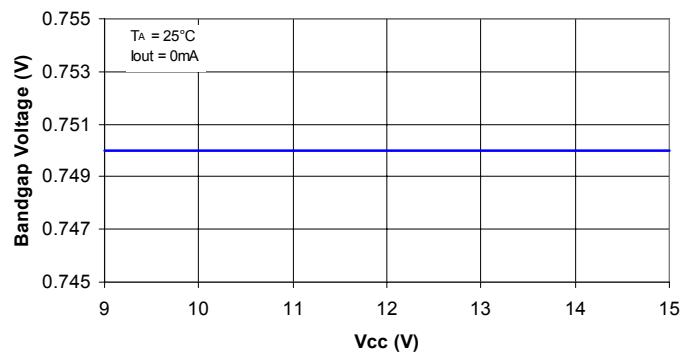
Bandgap Voltage vs Vcc
