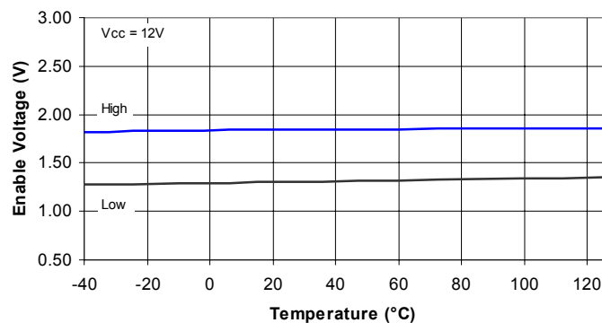
Enable Voltage vs Temperature
