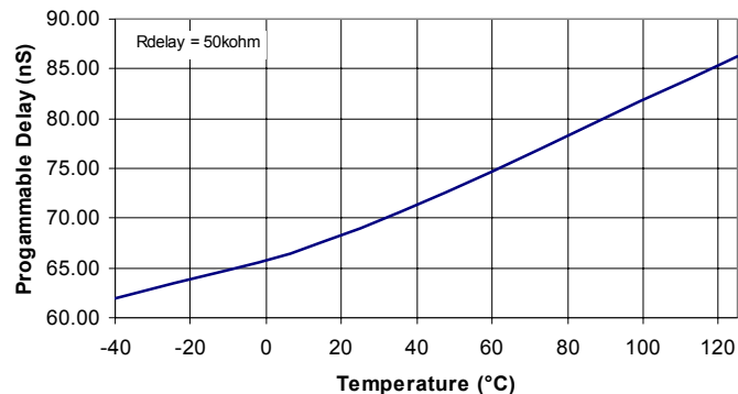
Programmable Delay vs Temperature
