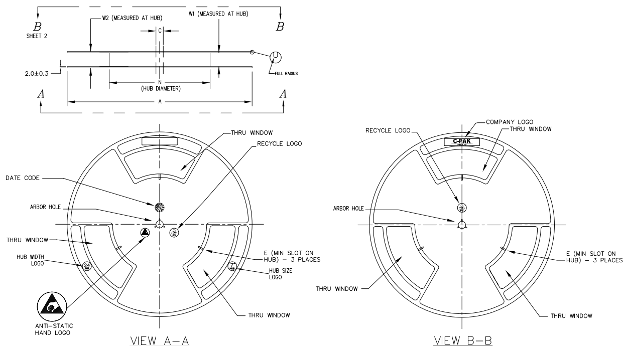
DIMENSIONS (MM)
