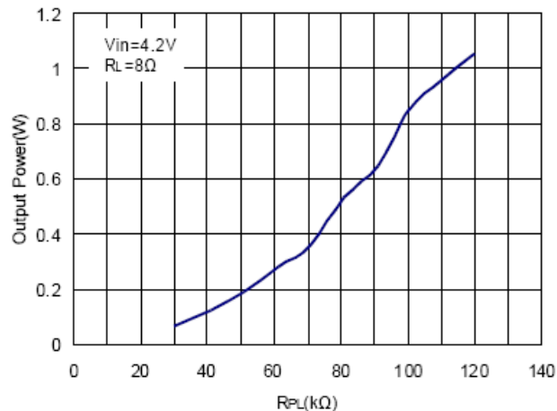
12. RPL VS Output Power
