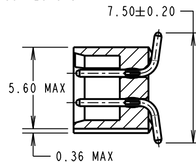
SECTION X-X
