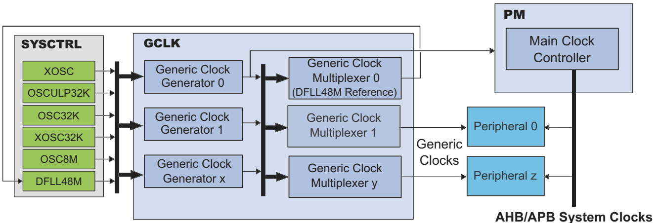
Figure 13-1. Clock distribution
