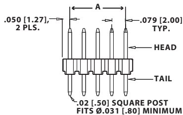
QUAD READOUT, STRAIGHT TAIL SHOWN
