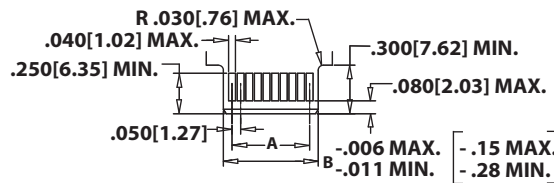
CARD LAYOUT
