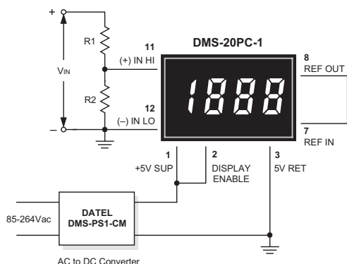
Figure 4. Input Attenuation Circuit
