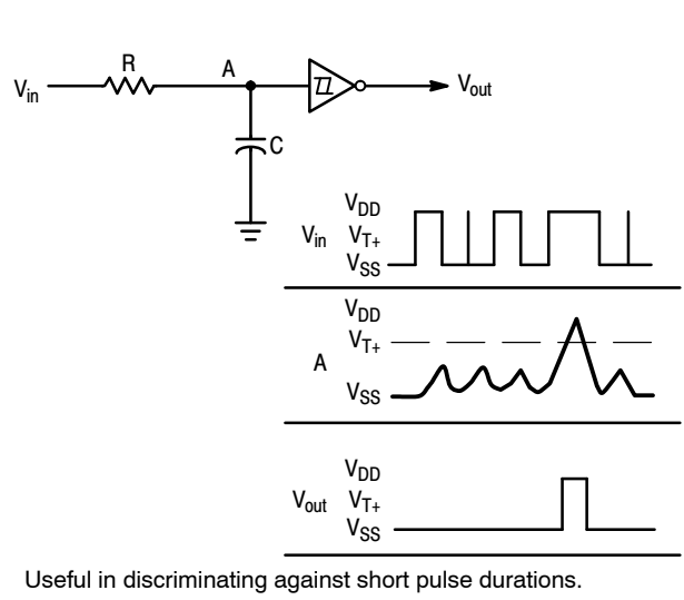
Figure 6. Integrator
