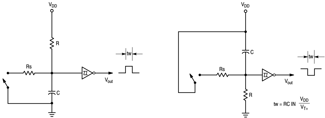
Figure 4. Monostable Multivibrator
