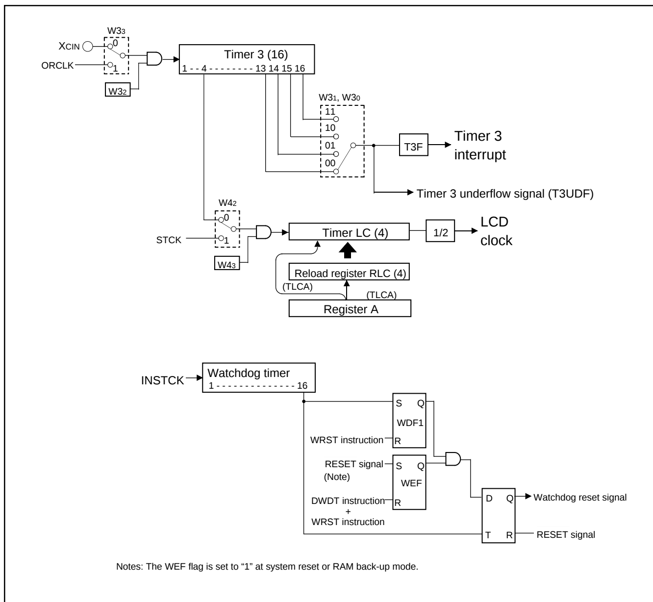
Fig. 23 Timer structure (2)
