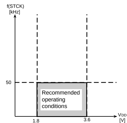
at quartz-crystal oscillation (One Time PROM version)
